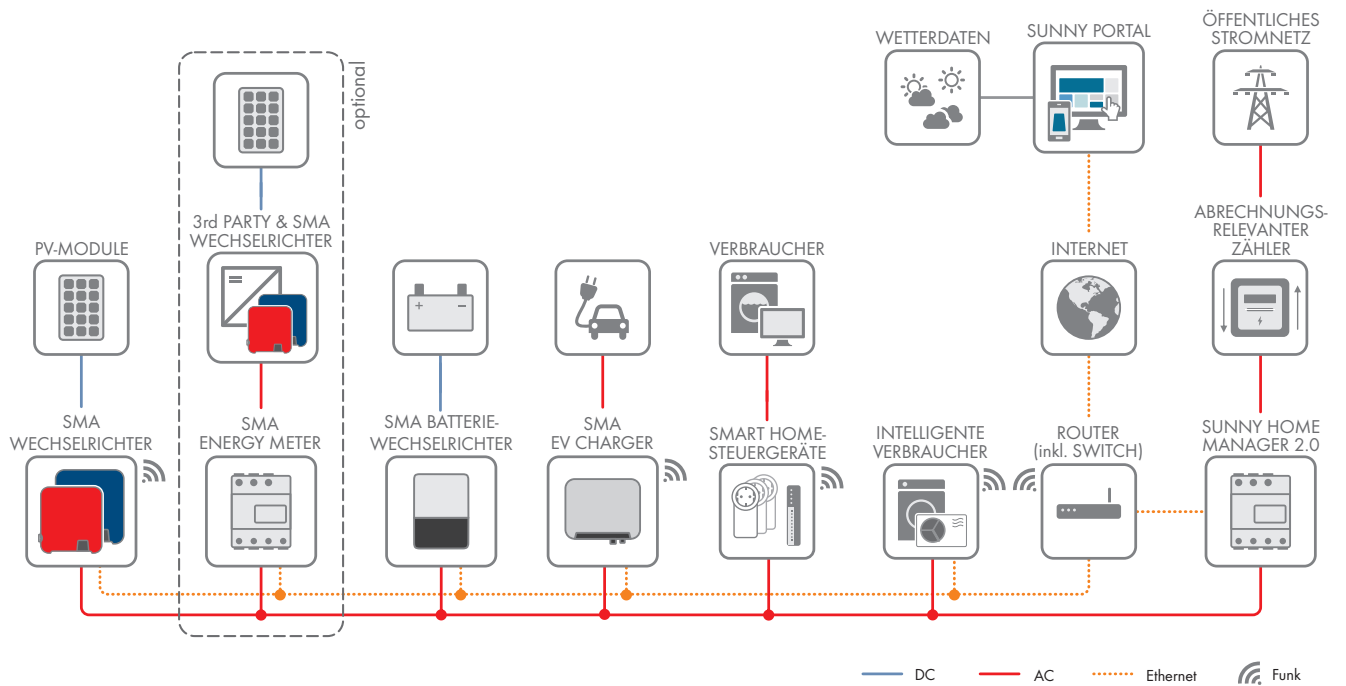
Figure 4: Topology showing SMA storage solutions and various controlled loads (general example)
